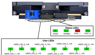
Figure 8 : Front Panel LEDs
