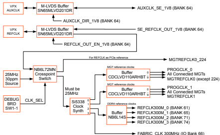
Figure 9 : Clock Topology
