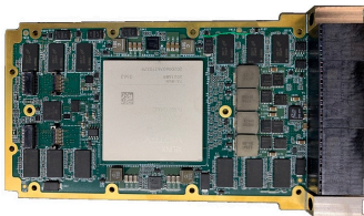
Figure 2 : ADM-VPX3-9V2 Top View
