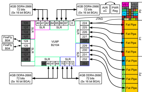
Figure 4 : ADM-VPX3-9V2 VU9P Block Diagram
