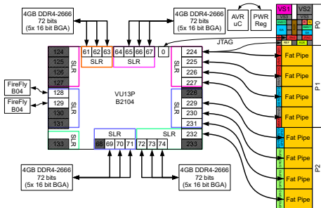
Figure 5 : ADM-VPX3-9V2 VU13P Block Diagram
